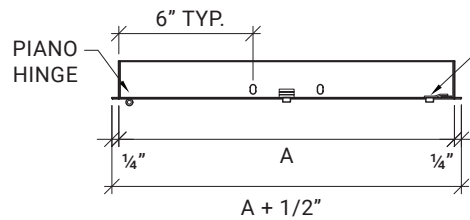
SECTION DETAIL
