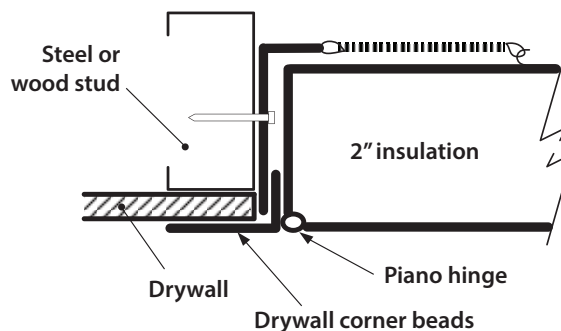
RECOMMENDED WALL INSTALLATION PROCEDURE FOR 1 HOUR RATING
