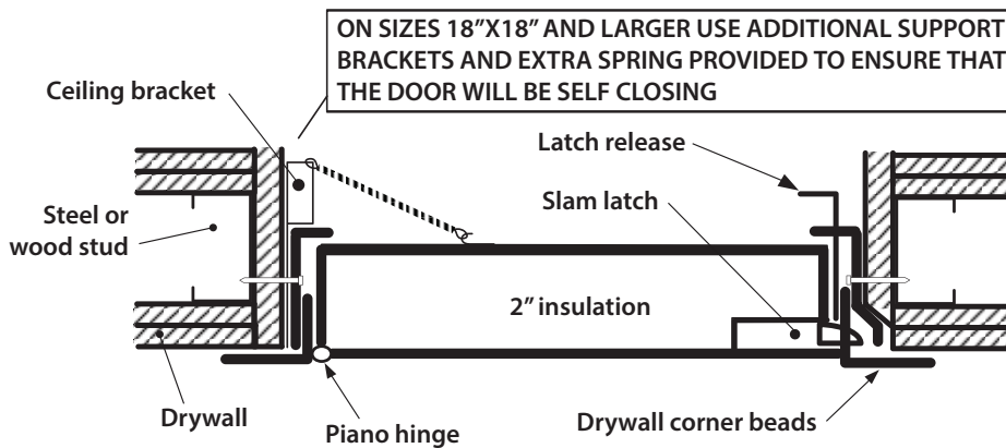
RECOMMENDED CEILING INSTALLATION PROCEDURE FOR 1 HOUR RATING
