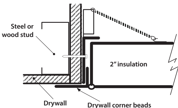
RECOMMENDED CEILING INSTALLATION PROCEDURE FOR 1 HOUR RATING
