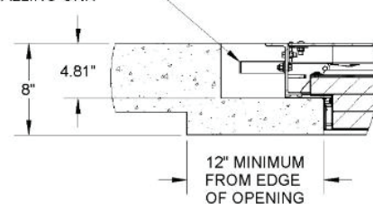
2-HR CAST IN DETAIL
