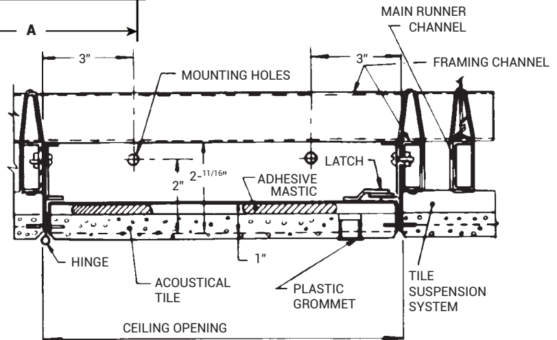
SECTION DETAIL
