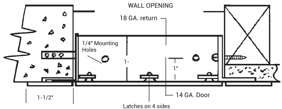
SECTION DETAIL
