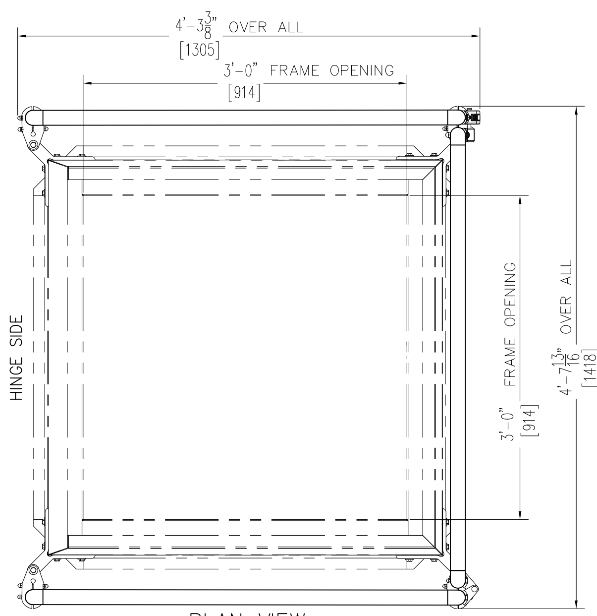
PLAN VIEW SHOWN WITHOUT COVER
