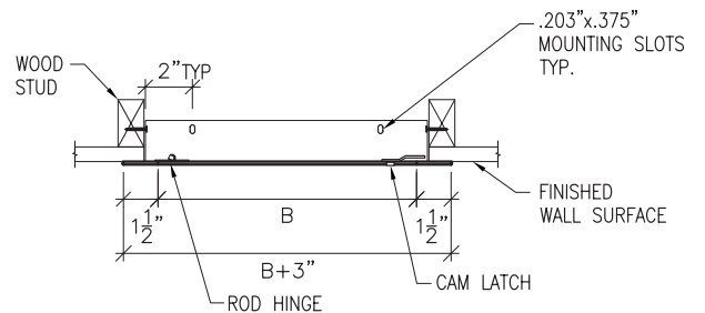
Section Detail
